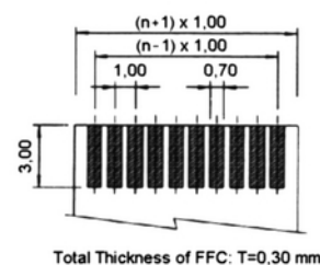
Recommended Flexible Flat Cable (FFC)
