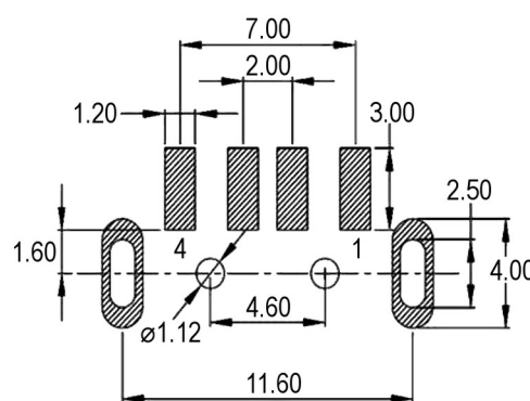
Recommended PCB Layout Component Side
