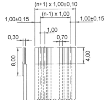
Recommended FFC-Dimensions
