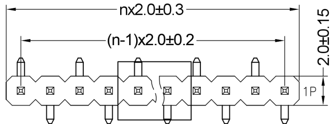
Layout B1
