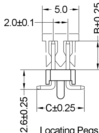
Locating Pegs Option -10-
