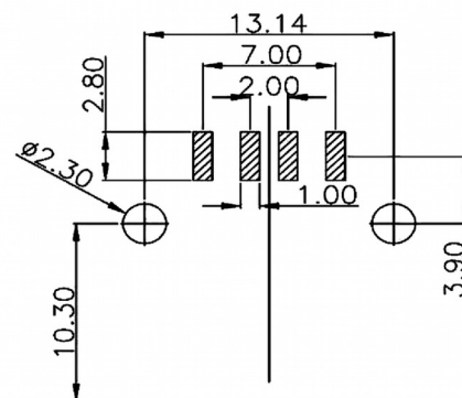
RECOMMENDED P. C. B. PATTERN LAYOUT
