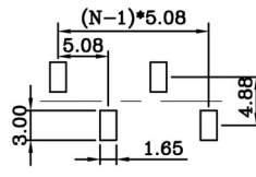
RECOMMENDED PCB LAYOUT (B1 Type)
