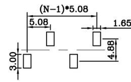
RECOMMENDED PCB LAYOUT (B2 Type)
